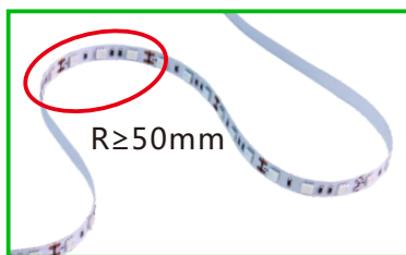
Bend(Right)
